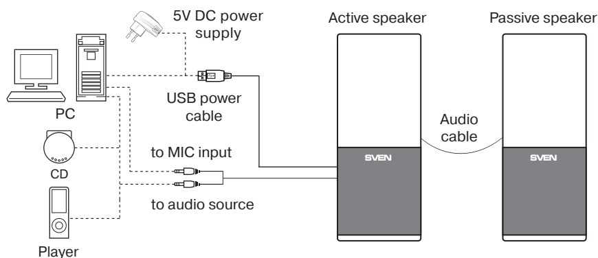
Fig. 2. Connection diagram
