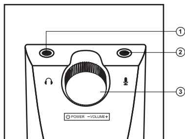
Fig. 1. Control panel
